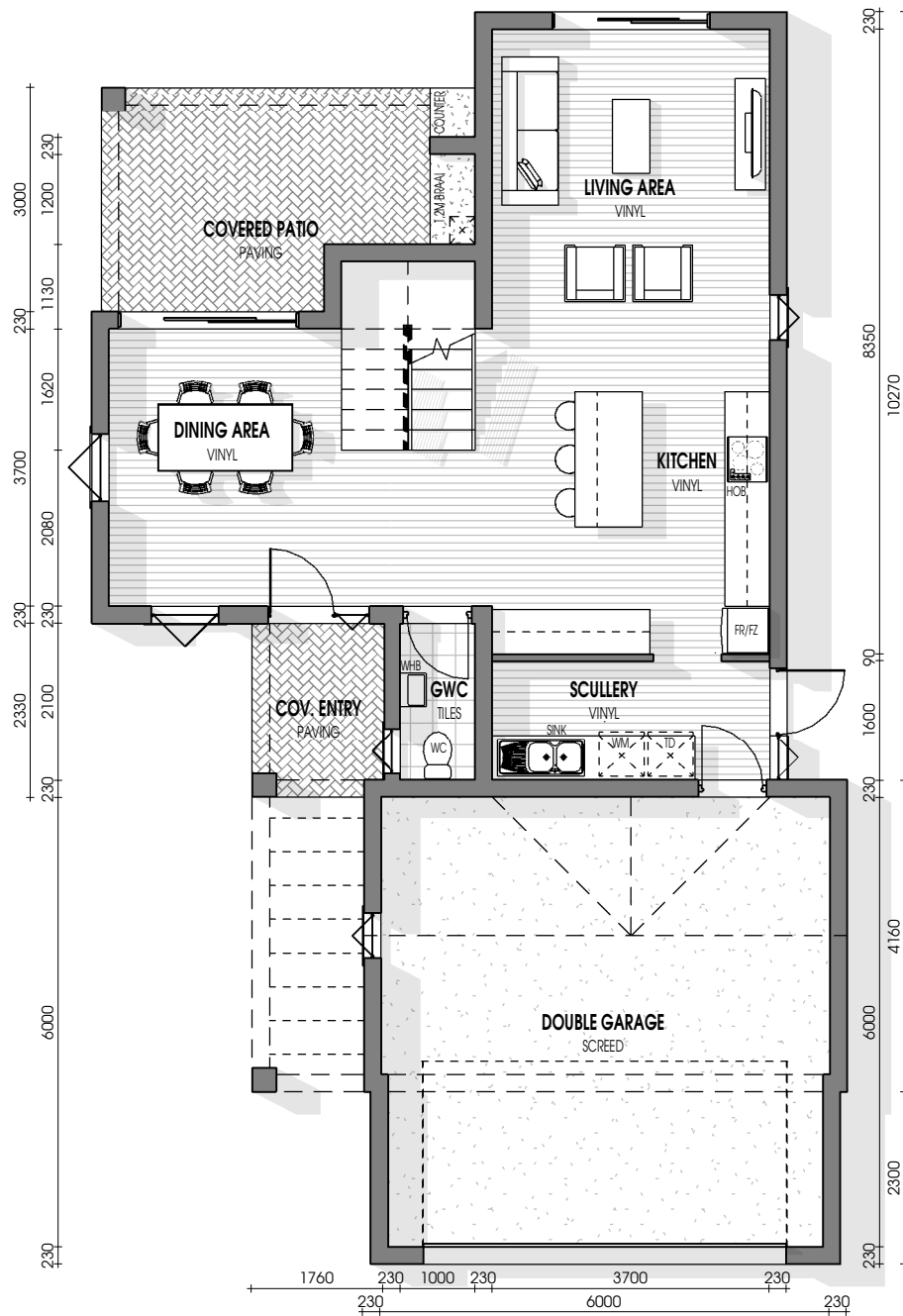
GROUND FLOOR Scale 1 : 100
