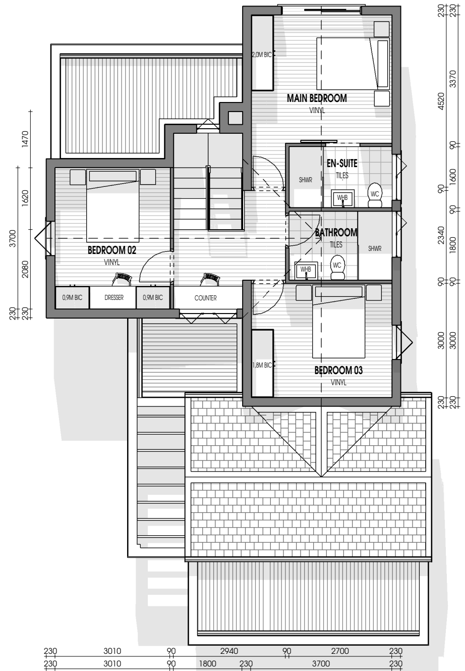
FIRST FLOOR Scale 1 : 100
