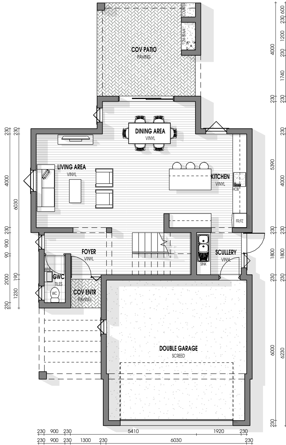
GROUND FLOOR Scale 1 : 100
