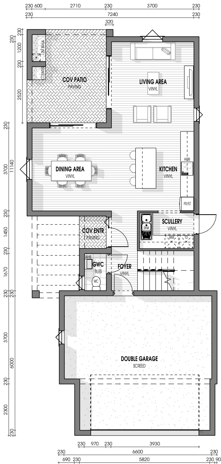
GROUND FLOOR Scale 1 : 100
