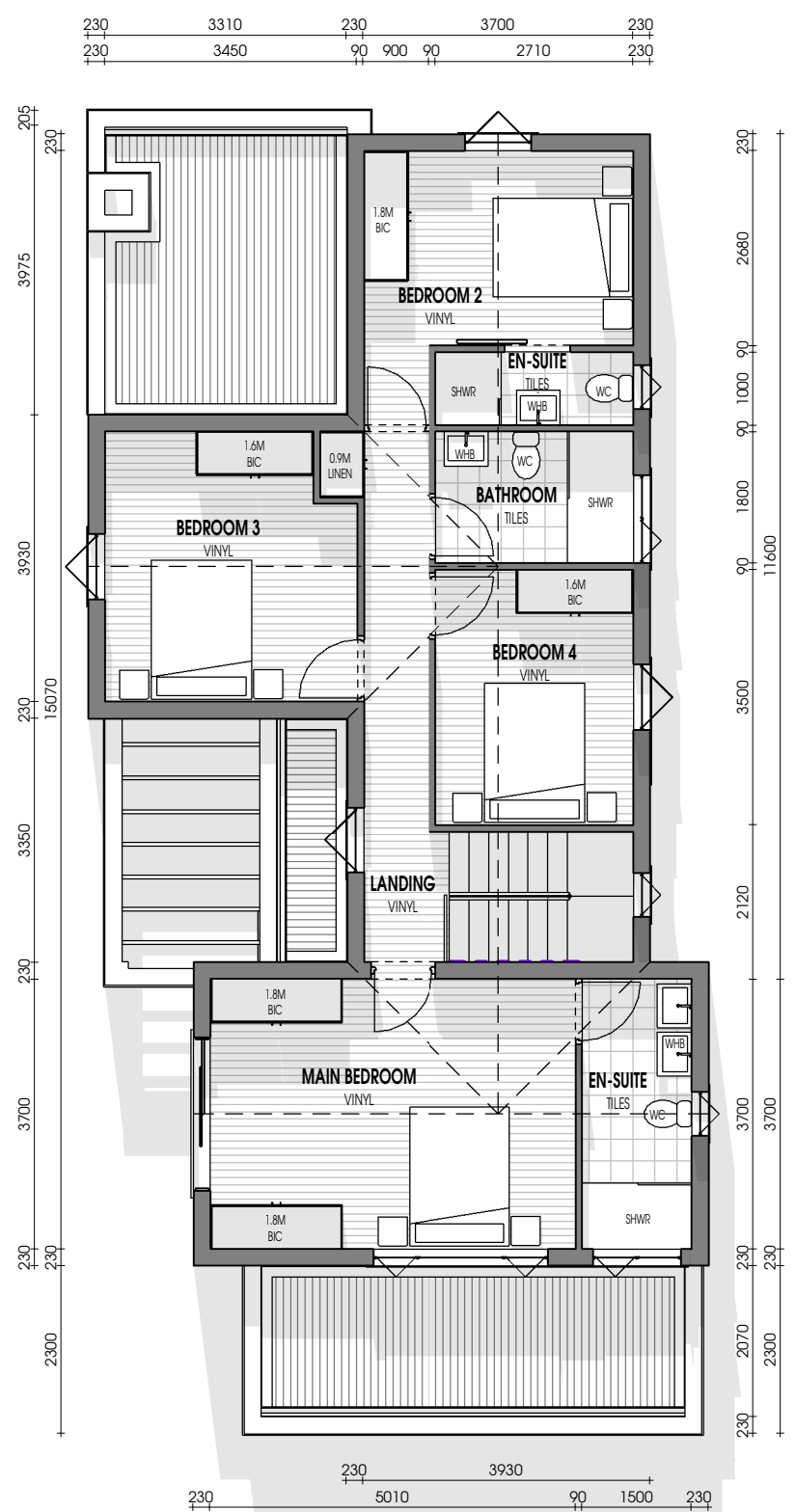
FIRST FLOOR Scale 1 : 100
