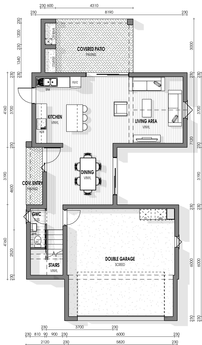
GROUND FLOOR Scale 1 : 100
