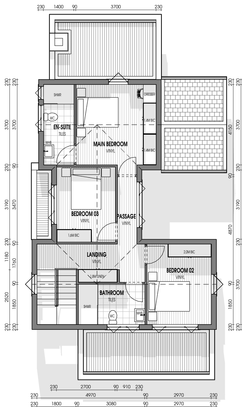
FIRST FLOOR Scale 1 : 100
