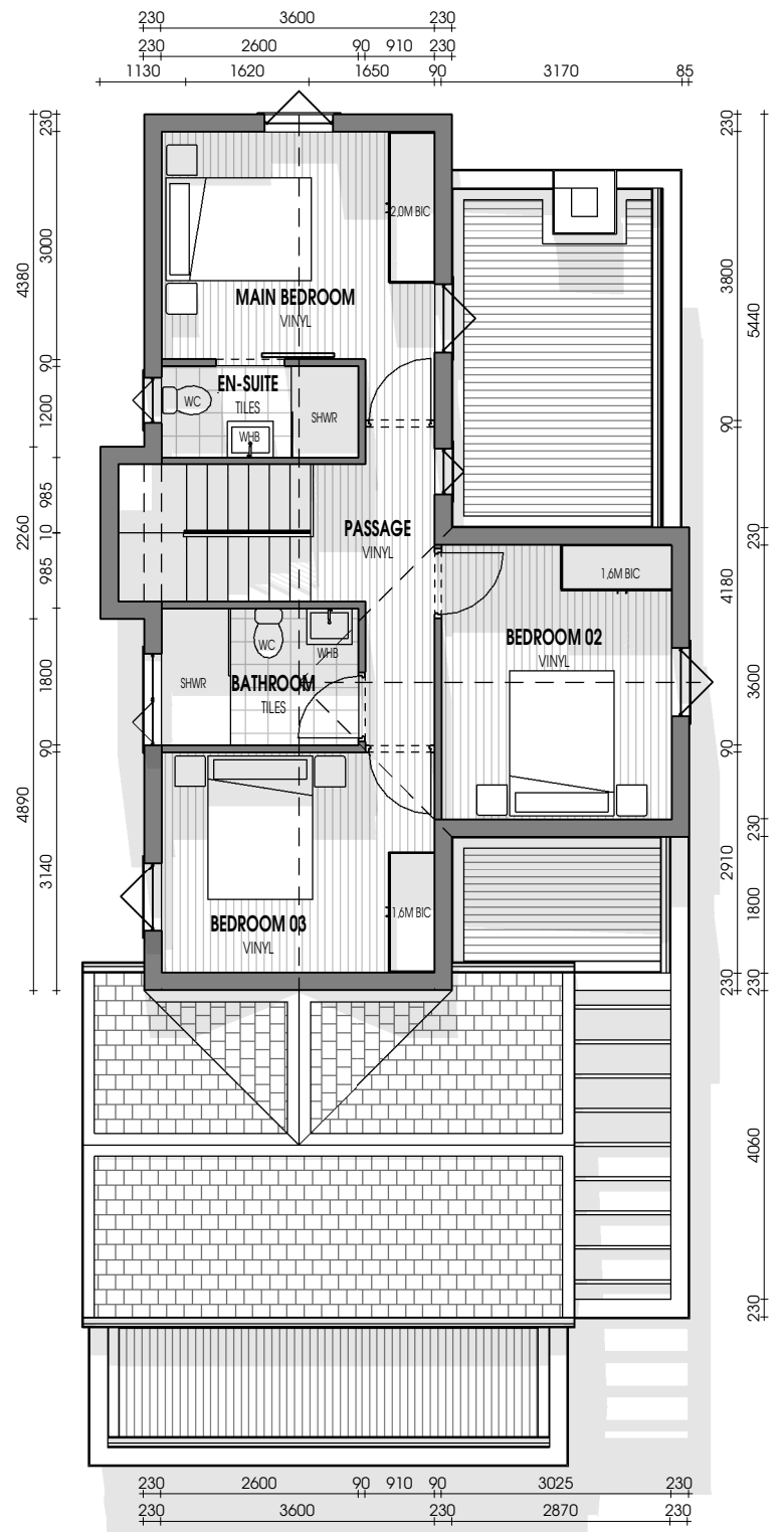
FIRST FLOOR Scale 1 : 100
